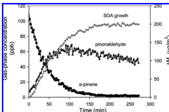
Figure 12. Time evolution of \alpha -pinene and pinonaldehyde from \alpha -pinene photo-oxidation as measured by PTR-MS in a reaction-chamber experiment. Also shown is the corresponding secondary organic aerosol (SOA) growth curve, as measured by aerosol mass spectrometry. Reprinted with permission from ref 171. Copyright 2006 American Chemical Society.
