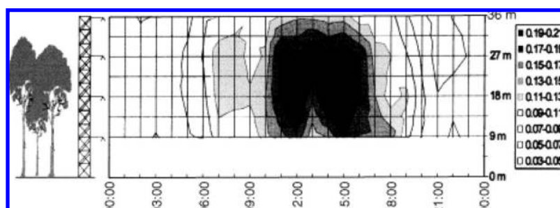
Figure 8. Contour plot of mean monoterpene concentration versus time of day (horizontal axis) and height above ground (vertical axis) from a study in a deciduous forest. Data are median values over 30 days. Concentration values are indicated in gray scale with steps of 0.02 ppbV. Reprinted with permission from ref 88. Copyright 2004 Elsevier.
