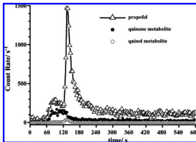
Figure 22. Real-time PTR-MS measurements of propofol and metabolite trace gas measurements for the first 10 min of breath sampling from a patient undergoing surgery. Reprinted with permission from ref 303. Copyright 2004 Elsevier.
